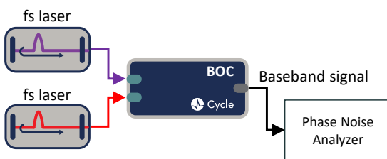
Timing jitter characterization
