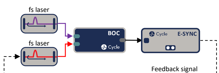
Femtosecond laser synchronization
