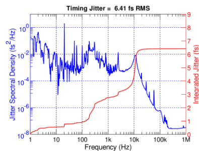
Out-of-loop timing jitter
